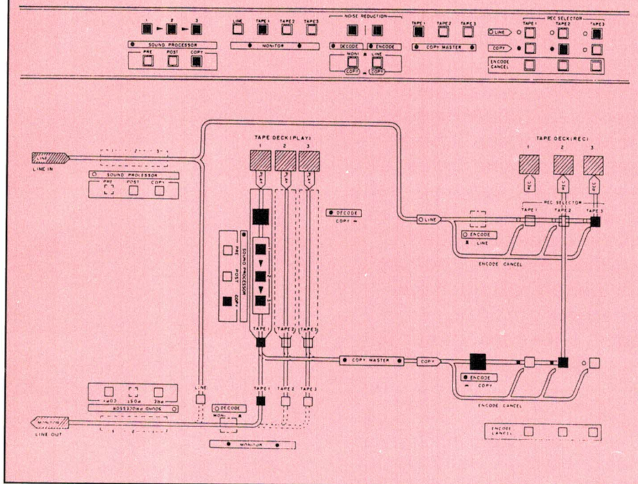
BLOCK DIAGRAM
